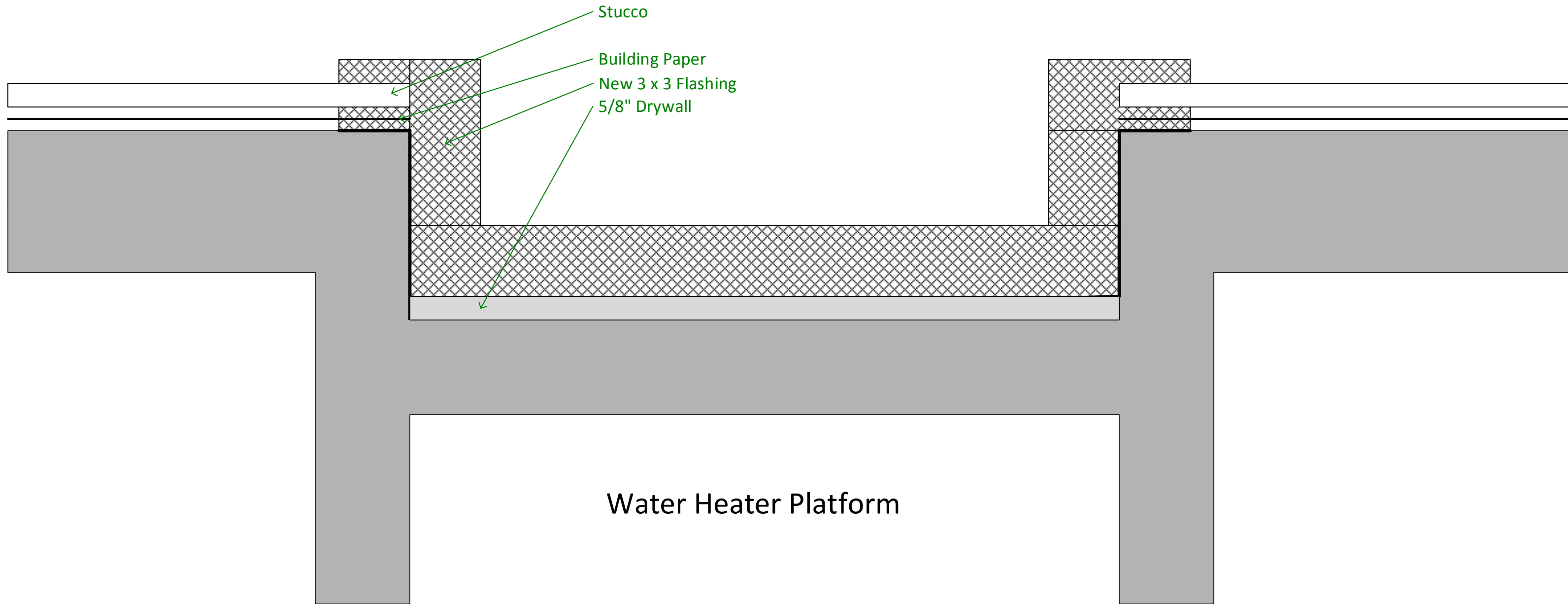
WATER HEATER DOOR – NEW SHEET METAL DETAIL – TOP VIEW
